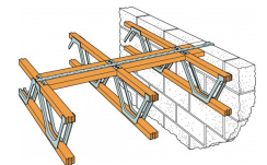
One strap at maximum 2m centres or as required by the building designer.
