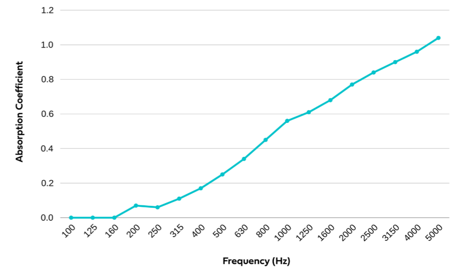
24mm Sound Absorption Coefficient
