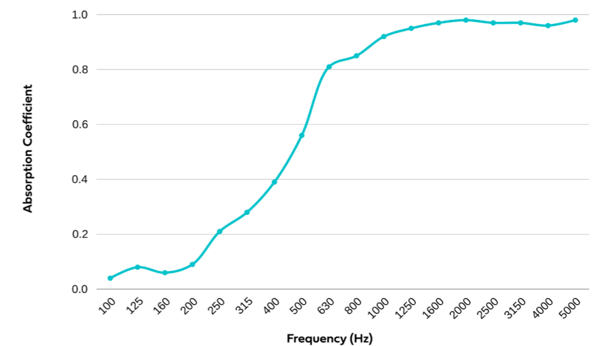
24mm Sound Absorption Coefficient
